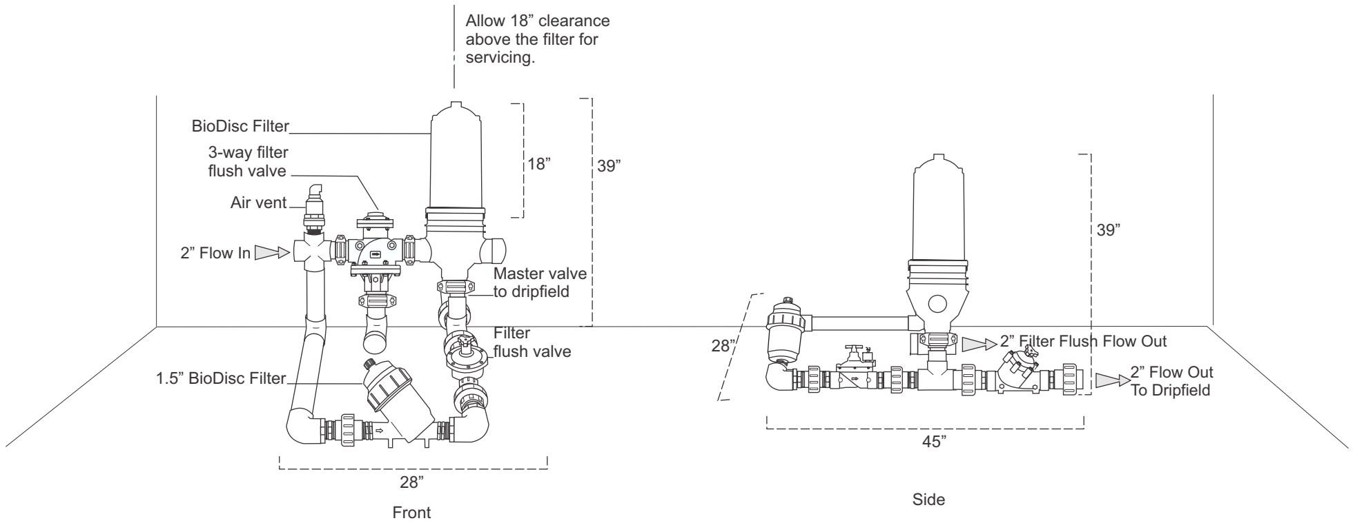
GEOFLOW Single Backwash Filter SUBSURFACE DRIP WHWBIODISC-1250FA-1
